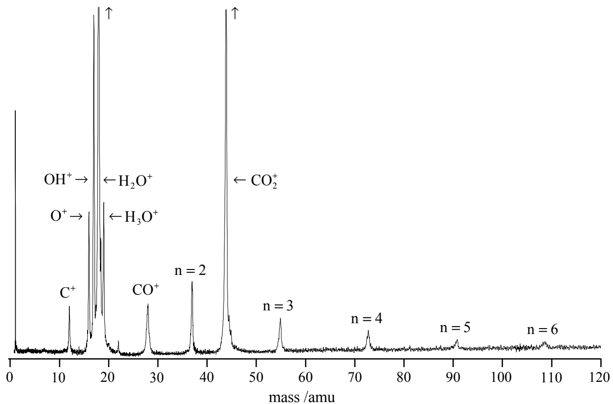
Figure 5. This spectrum highlights the presence of protonated water cluster ions. Note that the \text{H}_2\text{O}^+ and \text{CO}_2^+ peaks are off-scale. Conditions: 400 ML (25% \text{CO}_2 ), 2.4 mJ, average of 9 spots, 3 extractions for each spot.
