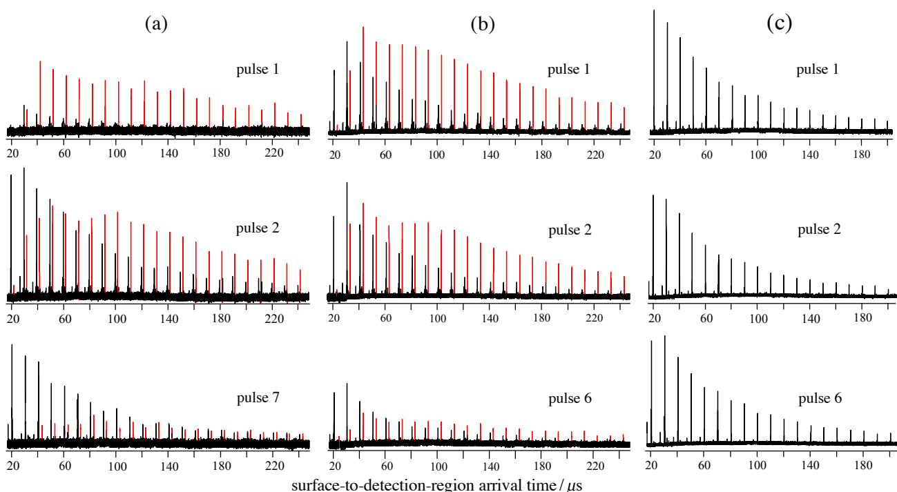
Figure 3. The horizontal axis is the arrival time at the detection region for material leaving the surface at t = 0 . The TOFMS is operated at 100 kHz, i.e. , individual spectra are recorded every 10\ \mu\text{s} (Figs. 4 and 5). (a) 500 ML (20% \text{CO}_2 ), 1.0 mJ: The first laser pulse liberates much more \text{CO}_2 (red) than \text{H}_2\text{O} (black). The second pulse liberates comparable amounts of \text{CO}_2 and \text{H}_2\text{O} . Pulse 7 liberates more \text{H}_2\text{O} than \text{CO}_2 . Keep in mind that the \text{H}_2\text{O}:\text{CO}_2 ratio for deposited material is 4:1. (b) 400 ML (25% \text{CO}_2 ), 1.2 mJ: The same general trend as in (a) is observed, though less dramatic. (c) 400 ML of \text{H}_2\text{O} (no \text{CO}_2 ), 1.2 mJ. Signal at 10\ \mu\text{s} is minuscule.
