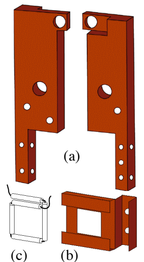
Figure 2. Exploded view of the substrate holder: (a) the electrically isolated copper blocks, (b) the folded copper plate that houses the substrate, and (c) the tantalum wire heater with ceramic sleeves, which is cemented to the back of the substrate holder. For resistive heating, the ends of the tantalum wires are connected to each of the electrically isolated blocks.
