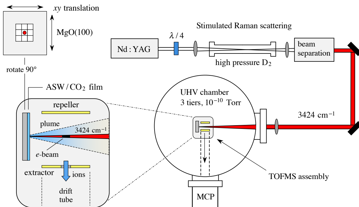
Figure 1. The UHV chamber is equipped with TOFMS, FTIR, Auger, and TPD. The TOFMS arrangement is indicated schematically. The second Stokes line ( 3424\text{ cm}^{-1} ) from stimulated Raman Scattering in high pressure \text{D}_2 gas excites the sample at normal incidence causing material to enter the gas phase. Ions are extracted at repetition rates up to 200 kHz. The black rectangle labeled e -beam indicates the portion of the ionized region that is extracted through the mesh aperture below it. Samples are irradiated in the nine areas indicated on the upper left to achieve signal averaging while maintaining single-pulse conditions.
