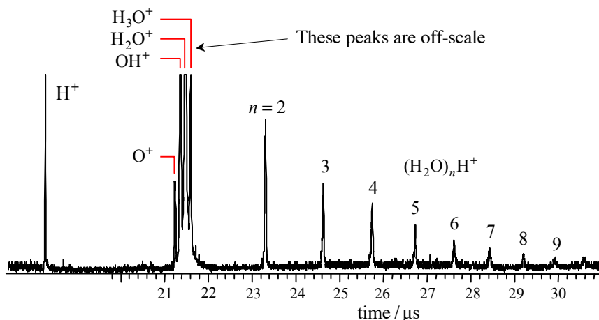
Figure 6. On rare occasion, relatively large cluster signals are observed, e.g., compare this spectrum to the one in Fig. 5. The sample is 400 ML of ASW; IR energy is 1.7 mJ.
